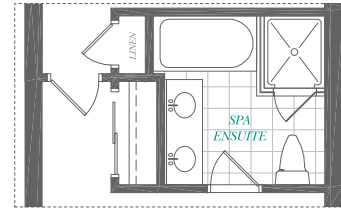
OPTIONAL UPGRADE SECOND FLOOR PARTIAL PLAN
