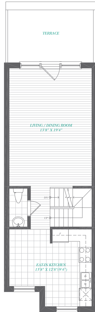
SECOND FLOOR
