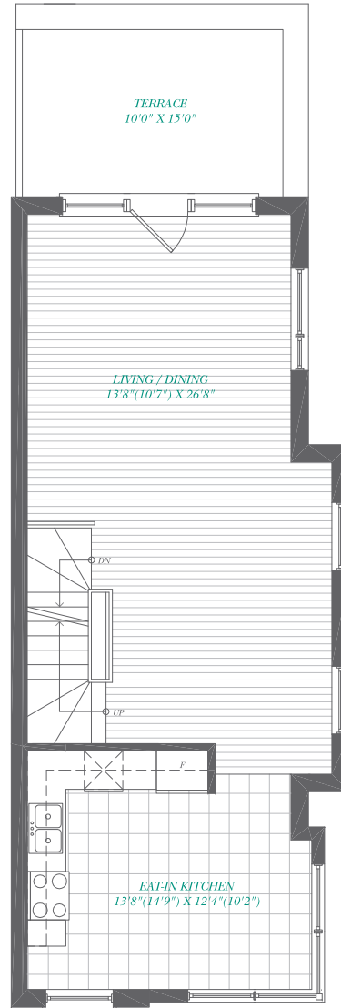
SECOND FLOOR
